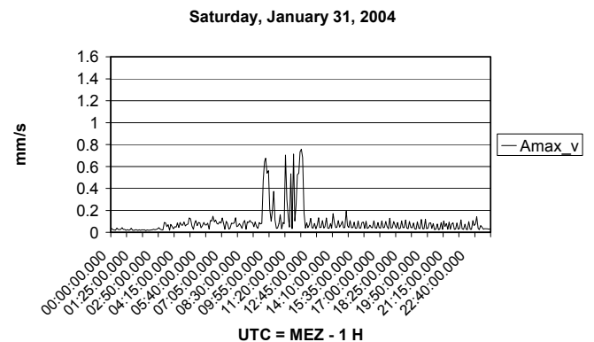
Figure 14. Floor vibrations for a typical Saturday.
