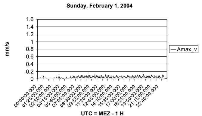
Figure 13. Floor vibrations for a typical Sunday.
