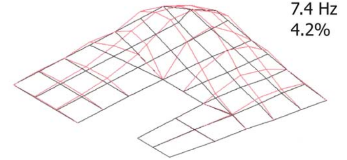
Figure 7. Mode 1, 2nd floor.
