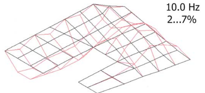
Figure 9. Mode 2, 2nd floor.
