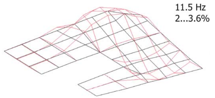
Figure 6. Mode 1, 1st floor
