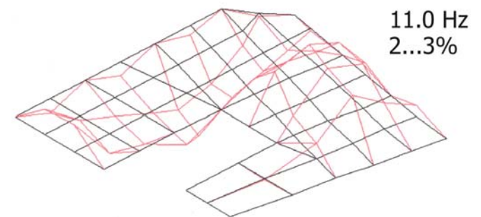
Figure 10. Mode 3, 2nd floor.
