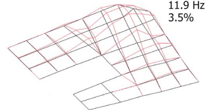
Figure 8. Mode 1, 3rd floor.
